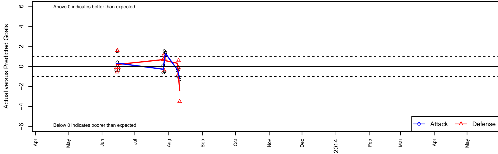
HSC Valencia B94 Dots are actual minus expected GF (blue circles) and GA (red triangles). Blue line is smoothed change in attack strength. Red is smoothed change in defense strength.
